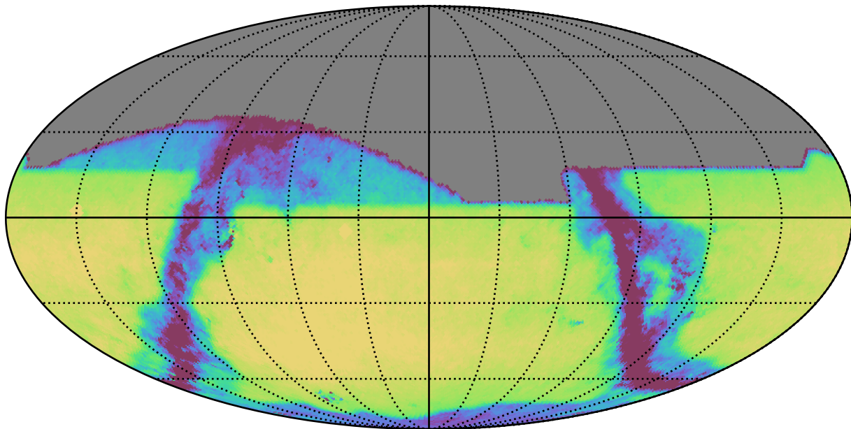
extra_ss_neo4_v3.4_10yrs All sky z band: Exgal_CoaddM5
