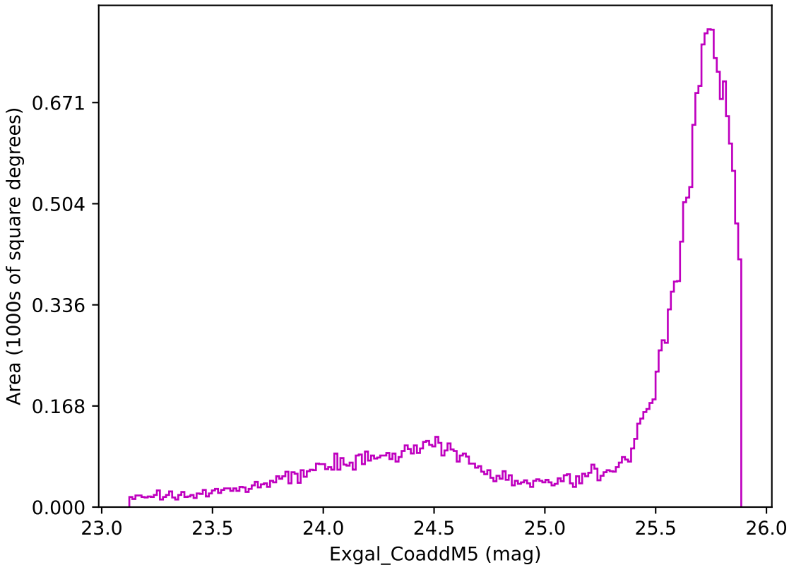
extra_ss_neo4_v3.4_10yrs All sky z band: Exgal_CoaddM5
