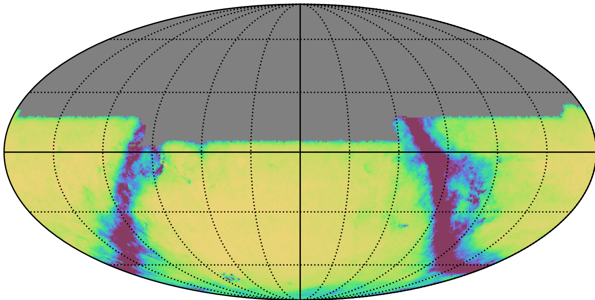
extra_ss_neo4_v3.4_10yrs All sky u band: Exgal_CoaddM5
