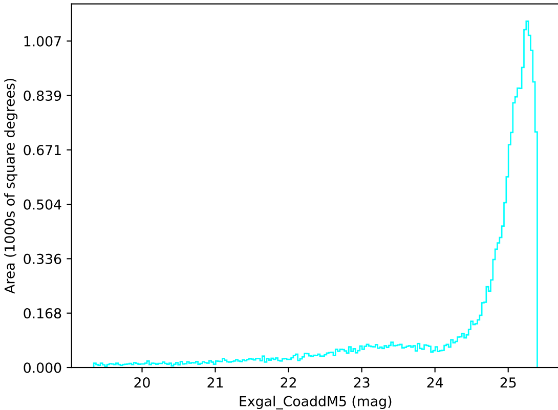
extra_ss_neo4_v3.4_10yrs All sky u band: Exgal_CoaddM5
