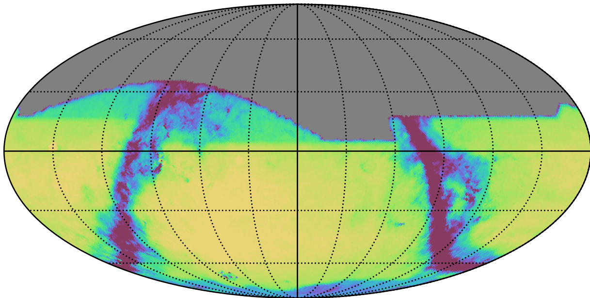
extra_ss_neo4_v3.4_10yrs All sky r band: Exgal_CoaddM5
