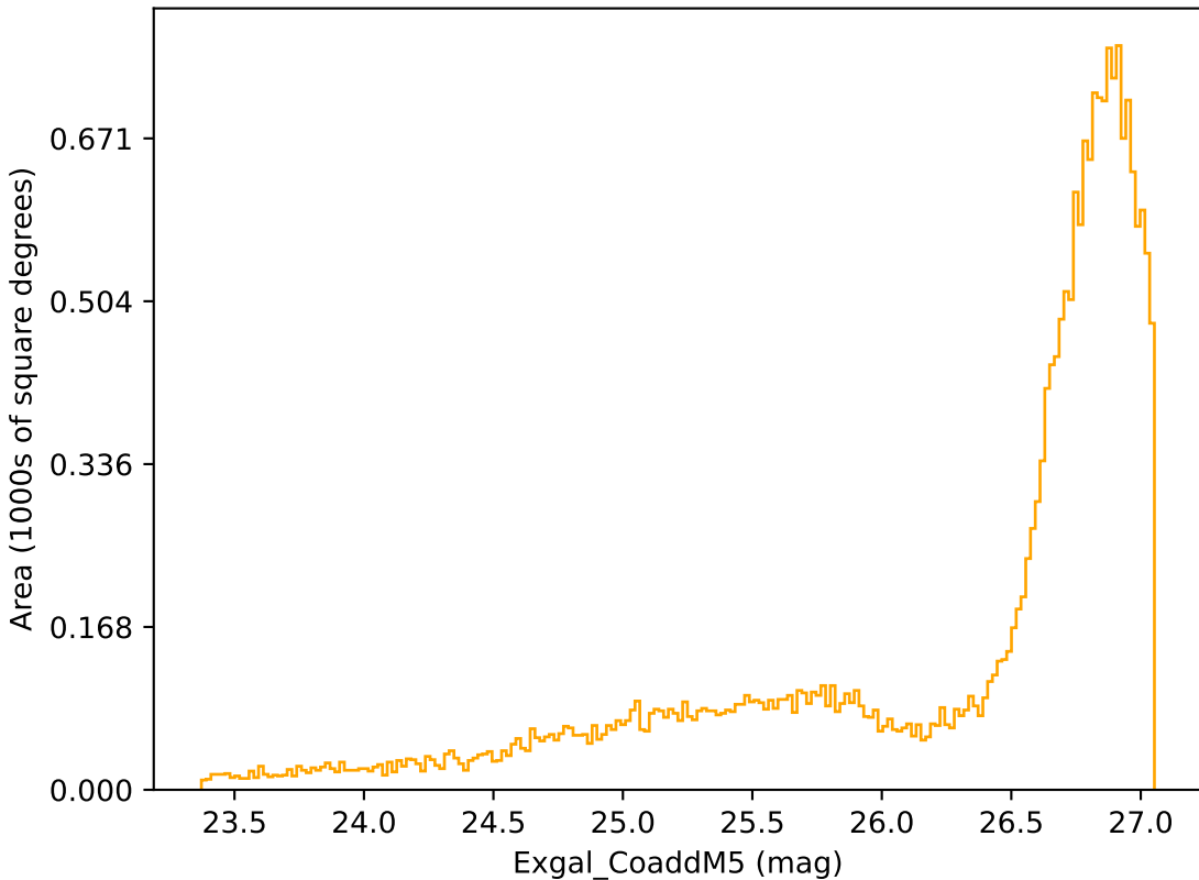
extra_ss_neo4_v3.4_10yrs All sky r band: Exgal_CoaddM5
