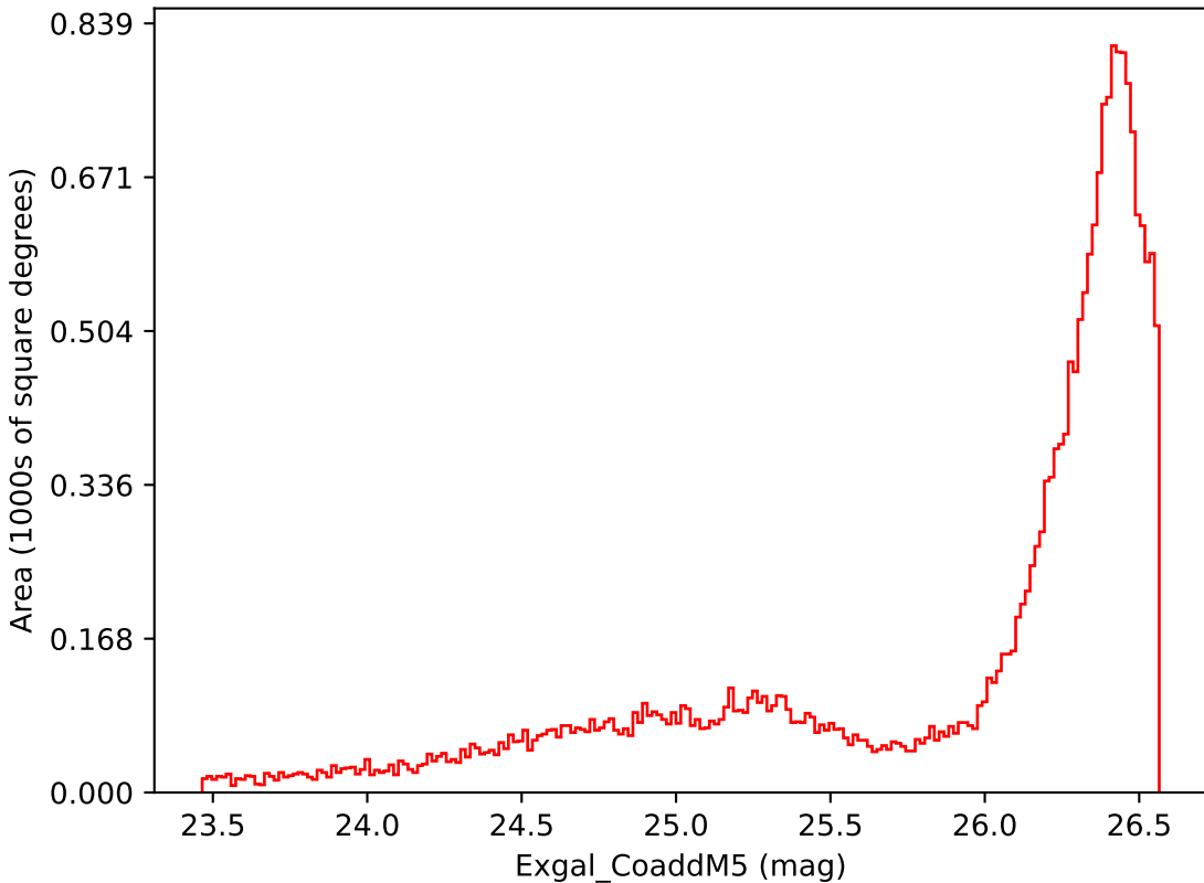
extra_ss_neo4_v3.4_10yrs All sky i band: Exgal_CoaddM5
