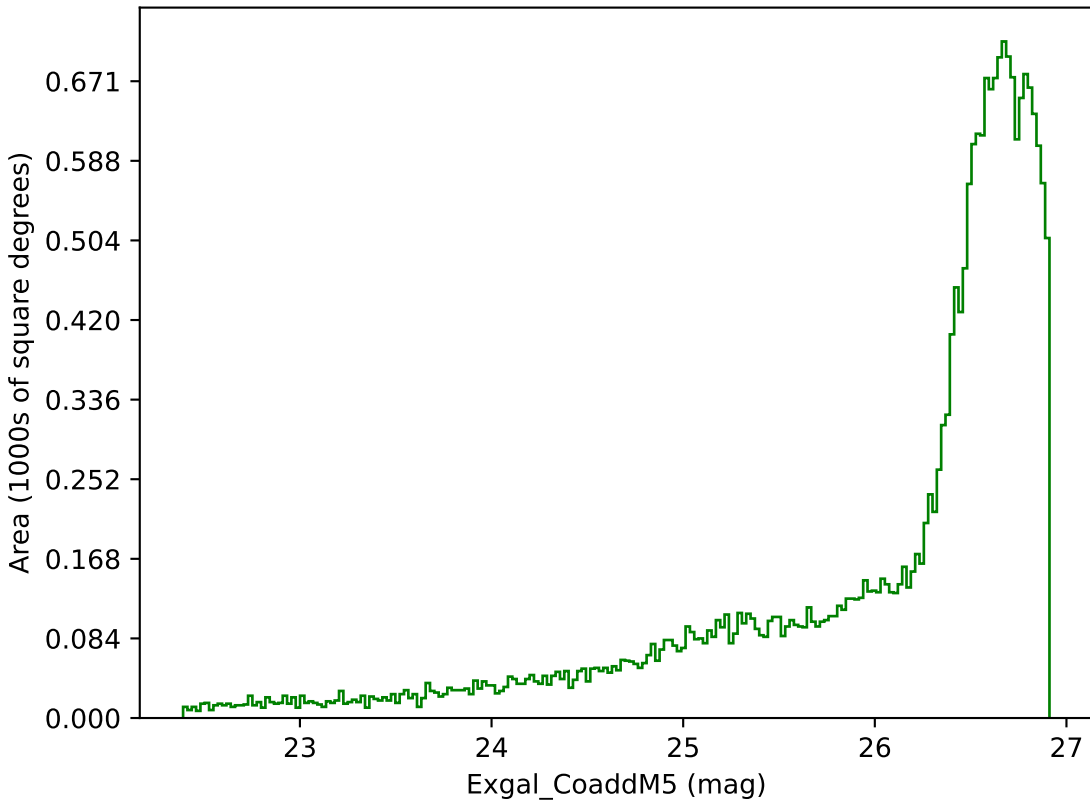
extra_ss_neo4_v3.4_10yrs All sky g band: Exgal_CoaddM5
