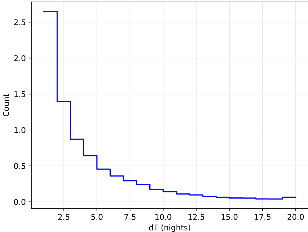
extra_ss_neo4_v3.4_10yrs WFD all bands: DeltaNight Histogram 1e6
