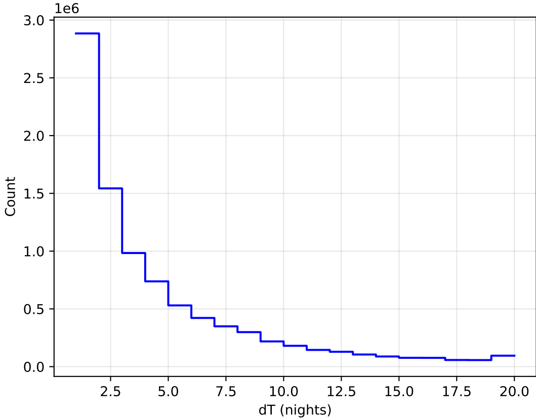
extra_ss_neo4_v3.4_10yrs All sky all bands: DeltaNight Histogram
