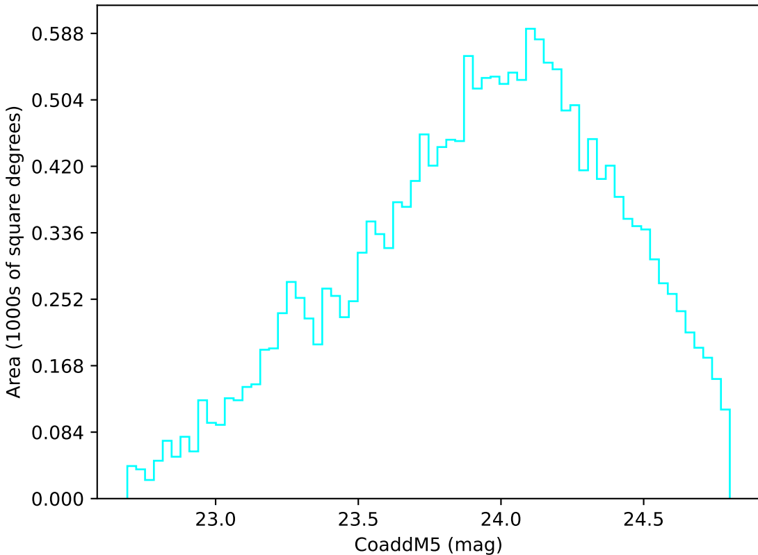
extra_ss_neo4_v3.4_10yrs Yr 3-4 u band: CoaddM5
