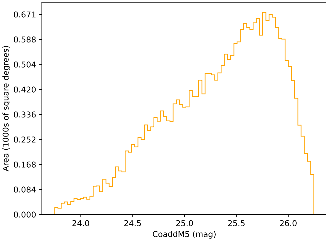
extra_ss_neo4_v3.4_10yrs Yr 3-4 r band: CoaddM5
