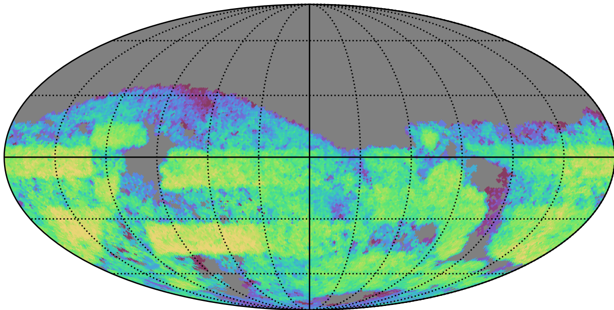
extra_ss_neo4_v3.4_10yrs Yr 3-4 g band: CoaddM5
