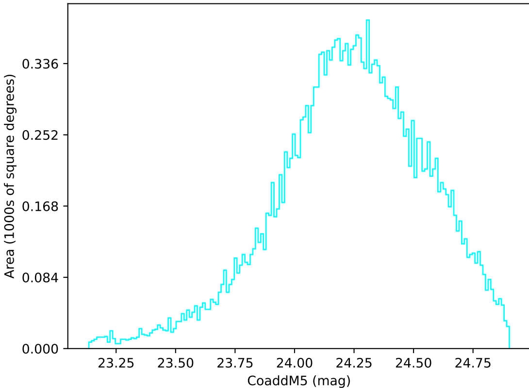
extra_ss_neo4_v3.4_10yrs Yr 1 u band: CoaddM5
