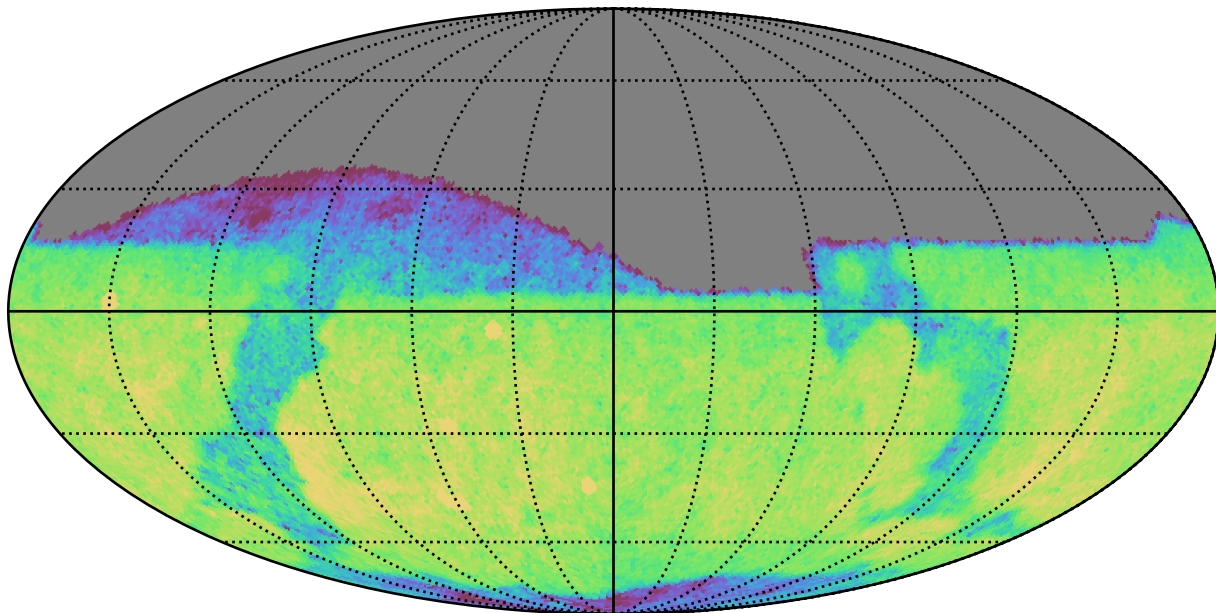
extra_ss_neo4_v3.4_10yrs Yr 1 r band: CoaddM5
