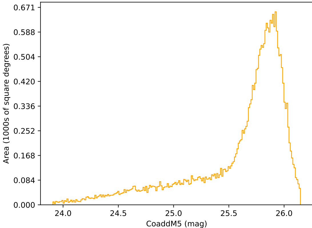
extra_ss_neo4_v3.4_10yrs Yr 1 r band: CoaddM5
