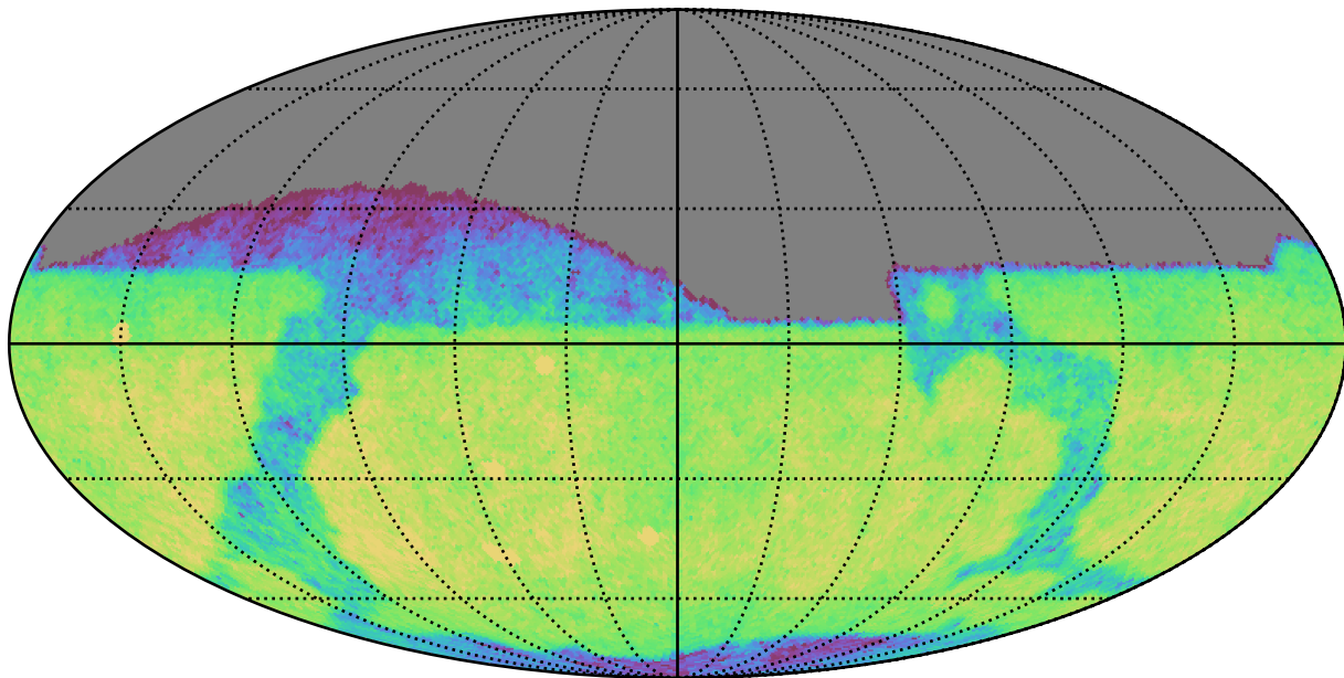
extra_ss_neo4_v3.4_10yrs Yr 1 i band: CoaddM5
