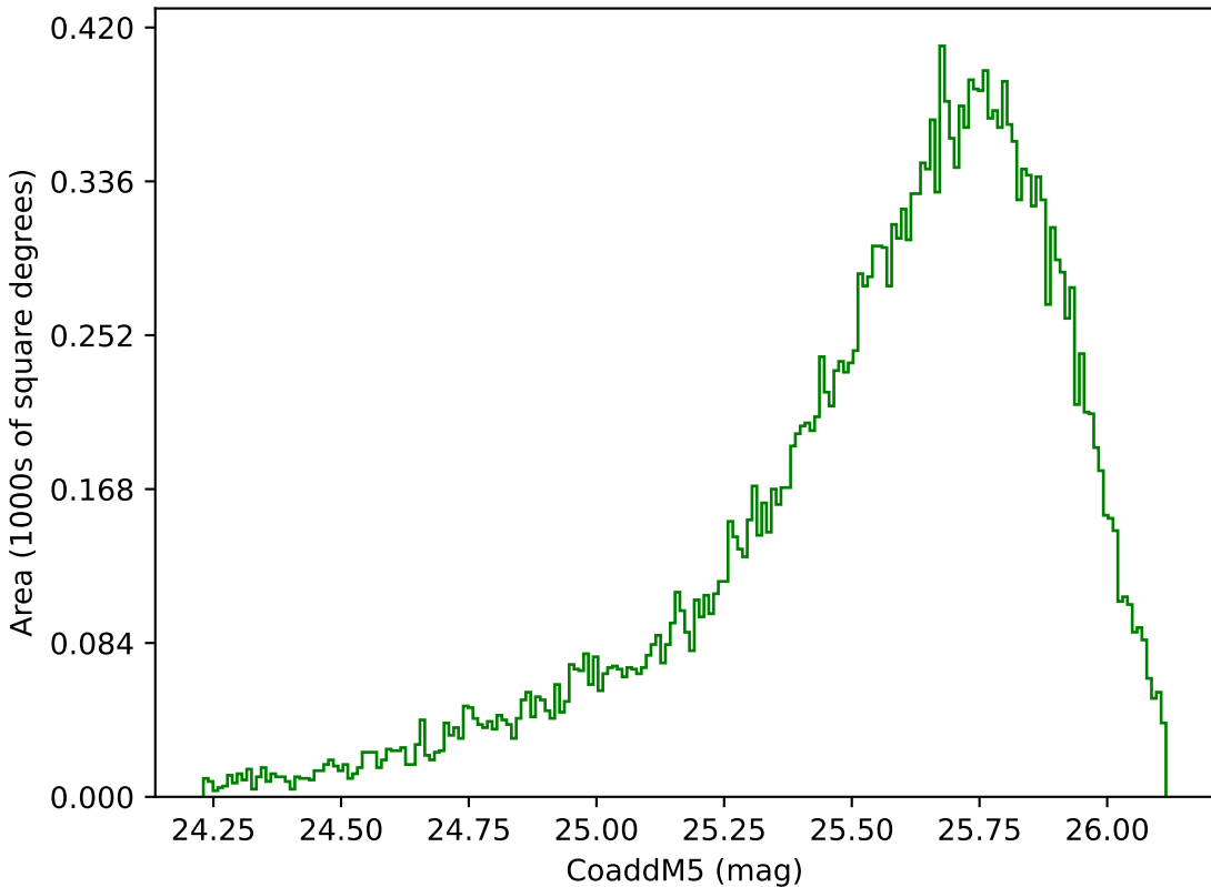
extra_ss_neo4_v3.4_10yrs Yr 1 g band: CoaddM5
