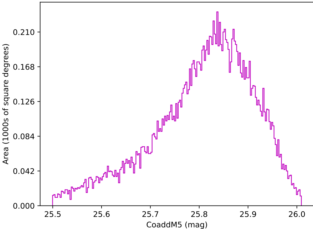
extra_ss_neo4_v3.4_10yrs WFD z band: CoaddM5
