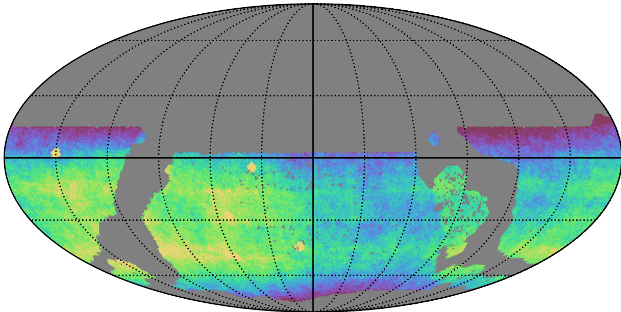
extra_ss_neo4_v3.4_10yrs WFD r band: CoaddM5
