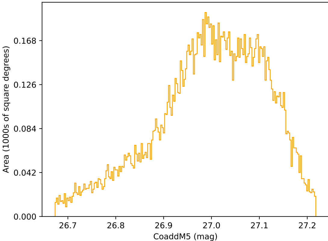
extra_ss_neo4_v3.4_10yrs WFD r band: CoaddM5
