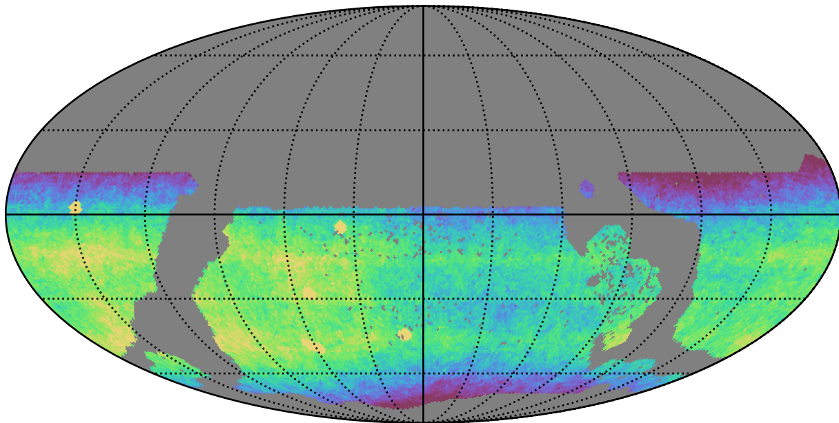
extra_ss_neo4_v3.4_10yrs WFD i band: CoaddM5
