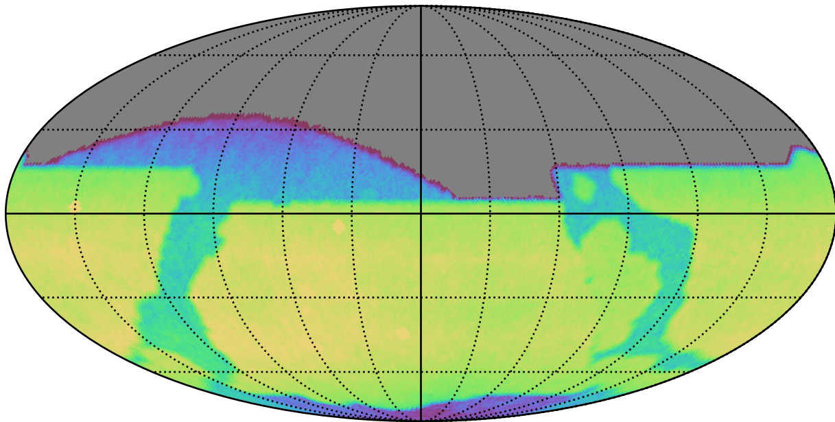
extra_ss_neo4_v3.4_10yrs All sky z band: CoaddM5
