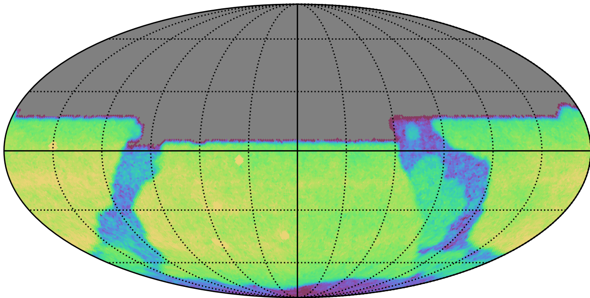
extra_ss_neo4_v3.4_10yrs All sky u band: CoaddM5
