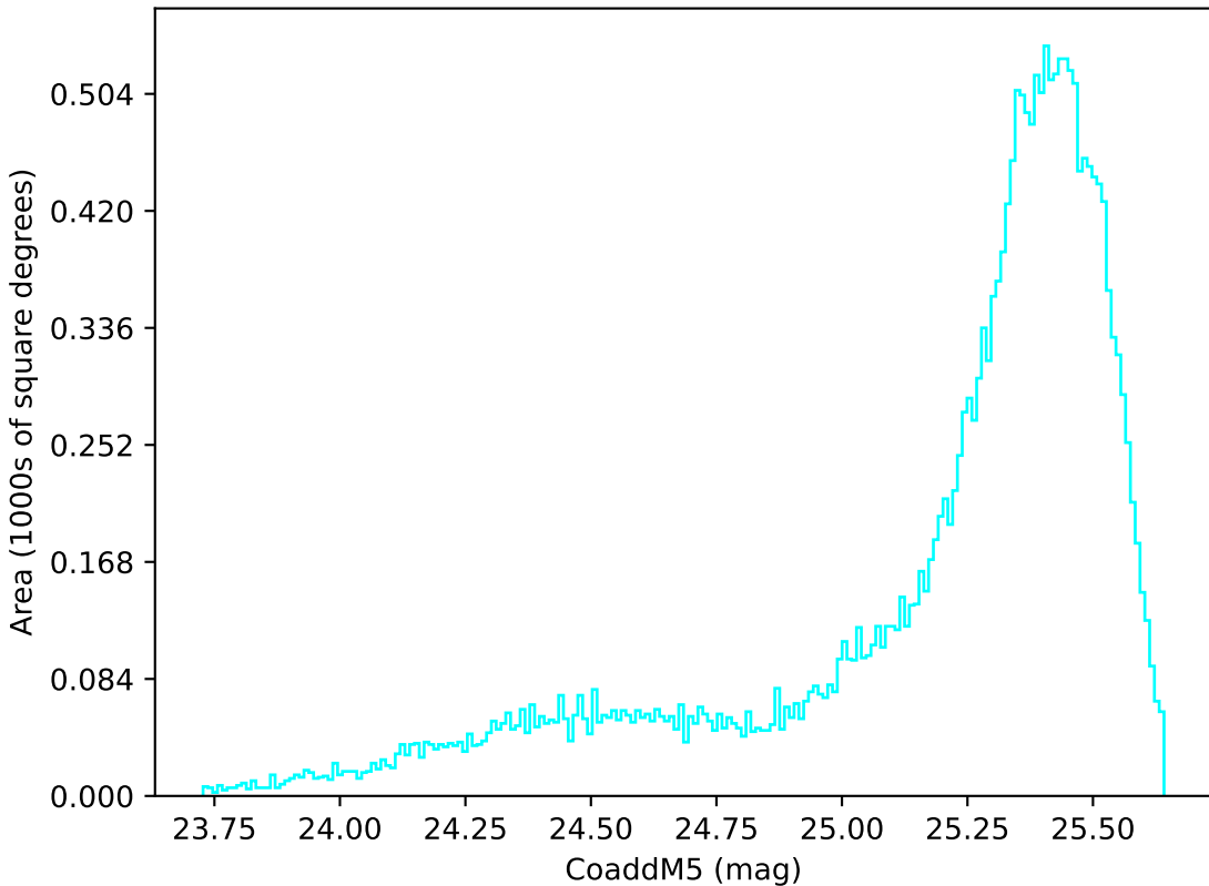
extra_ss_neo4_v3.4_10yrs All sky u band: CoaddM5
