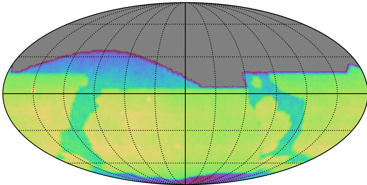
extra_ss_neo4_v3.4_10yrs All sky r band: CoaddM5
