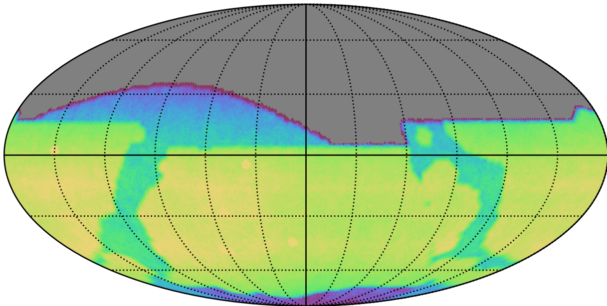
extra_ss_neo4_v3.4_10yrs All sky i band: CoaddM5
