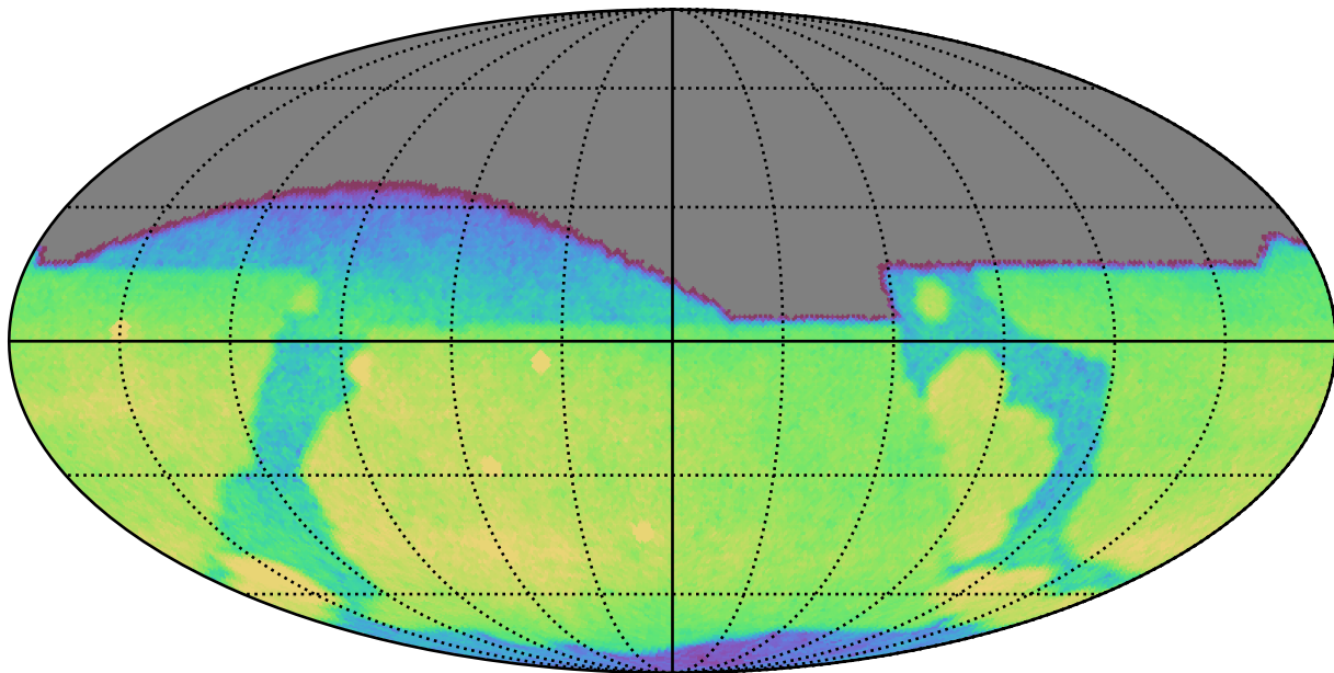
extra_ss_neo4_v3.4_10yrs All sky g band: CoaddM5
