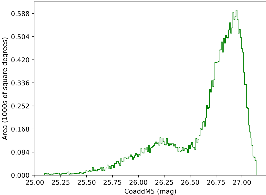
extra_ss_neo4_v3.4_10yrs All sky g band: CoaddM5
