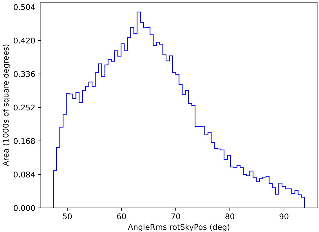
extra_ss_neo4_v3.4_10yrs WFD z band: AngleRms rotSkyPos
