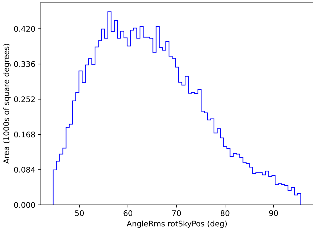
extra_ss_neo4_v3.4_10yrs WFD u band: AngleRms rotSkyPos
