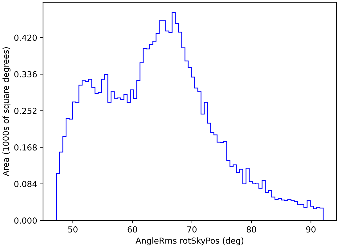
extra_ss_neo4_v3.4_10yrs WFD i band: AngleRms rotSkyPos
