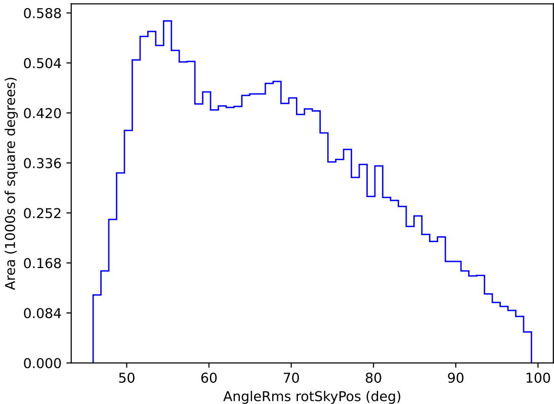
extra_ss_neo4_v3.4_10yrs WFD g band: AngleRms rotSkyPos
