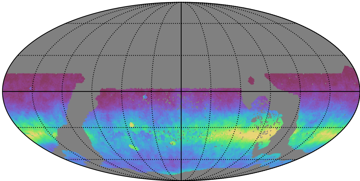
extra_ss_neo4_v3.4_10yrs WFD all bands: AngleRms rotSkyPos
