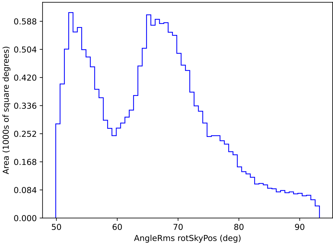
extra_ss_neo4_v3.4_10yrs WFD all bands: AngleRms rotSkyPos
