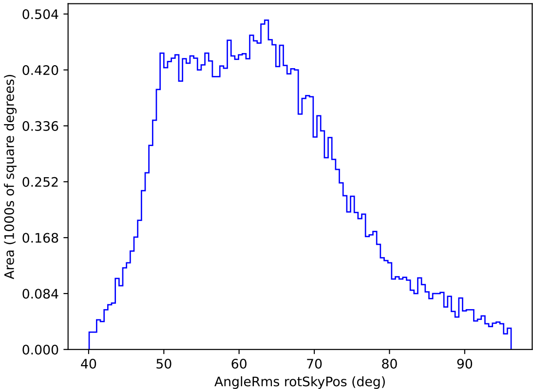
extra_ss_neo4_v3.4_10yrs All sky z band: AngleRms rotSkyPos
