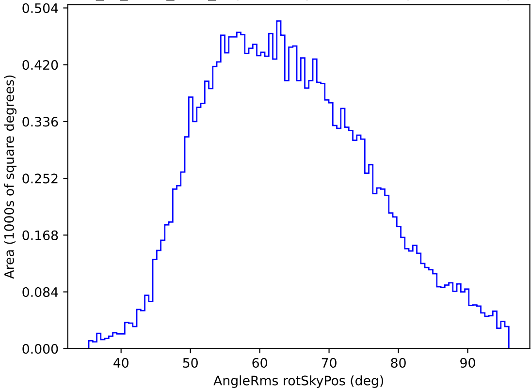
extra_ss_neo4_v3.4_10yrs All sky u band: AngleRms rotSkyPos
