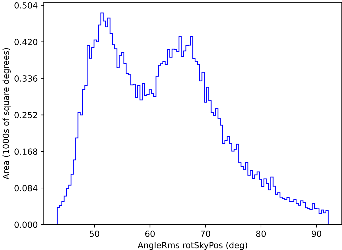
extra_ss_neo4_v3.4_10yrs All sky i band: AngleRms rotSkyPos
