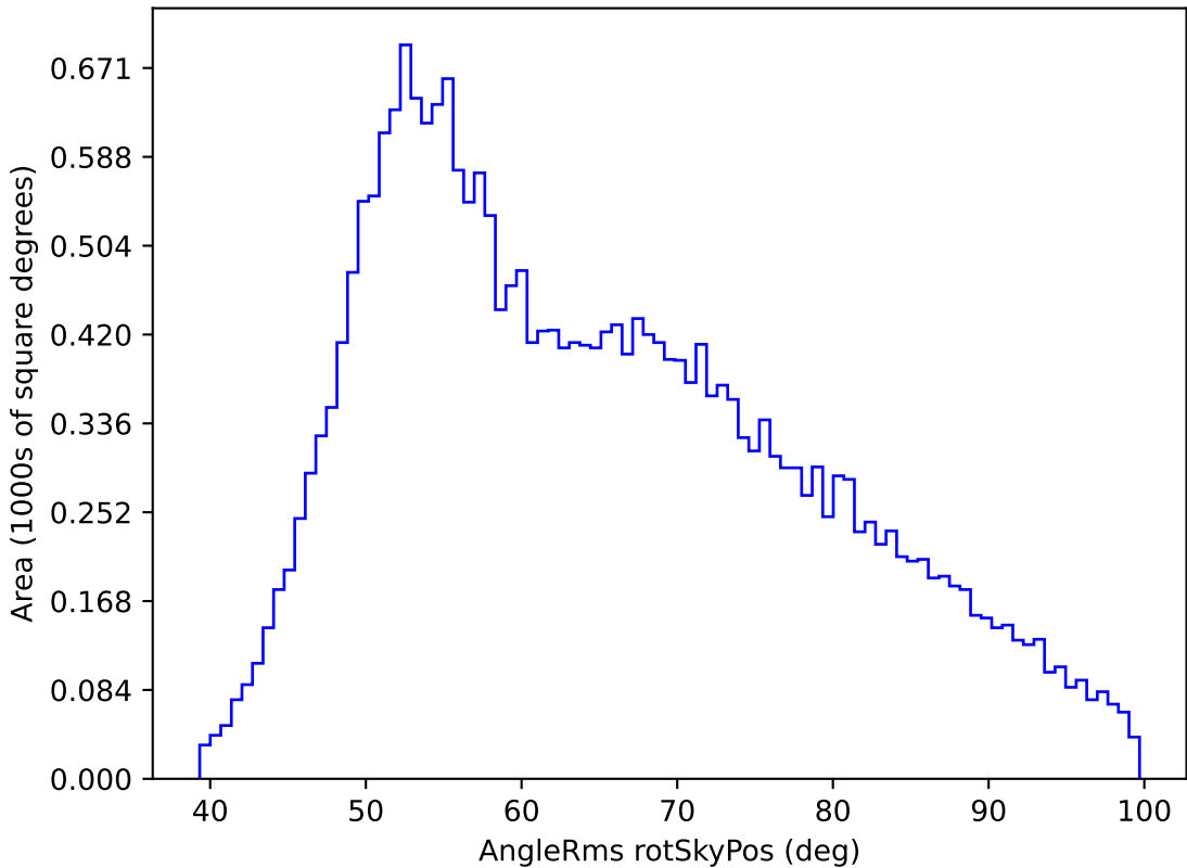
extra_ss_neo4_v3.4_10yrs All sky g band: AngleRms rotSkyPos
