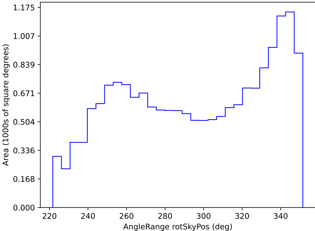
extra_ss_neo4_v3.4_10yrs WFD all bands: AngleRange rotSkyPos
