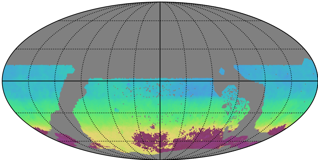
extra_ss_neo4_v3.4_10yrs WFD z band: AngleMean rotSkyPos
