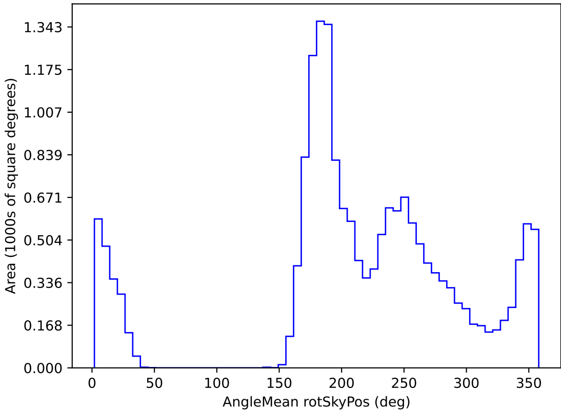
extra_ss_neo4_v3.4_10yrs WFD z band: AngleMean rotSkyPos
