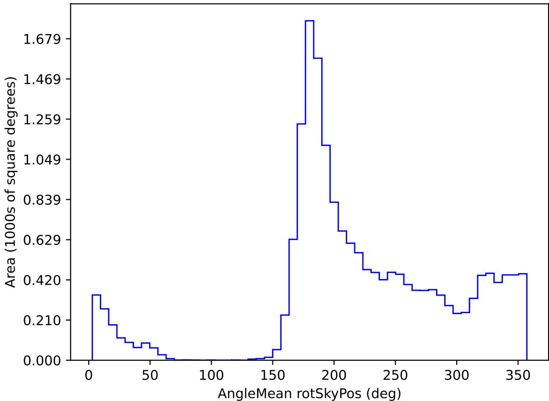
extra_ss_neo4_v3.4_10yrs WFD u band: AngleMean rotSkyPos
