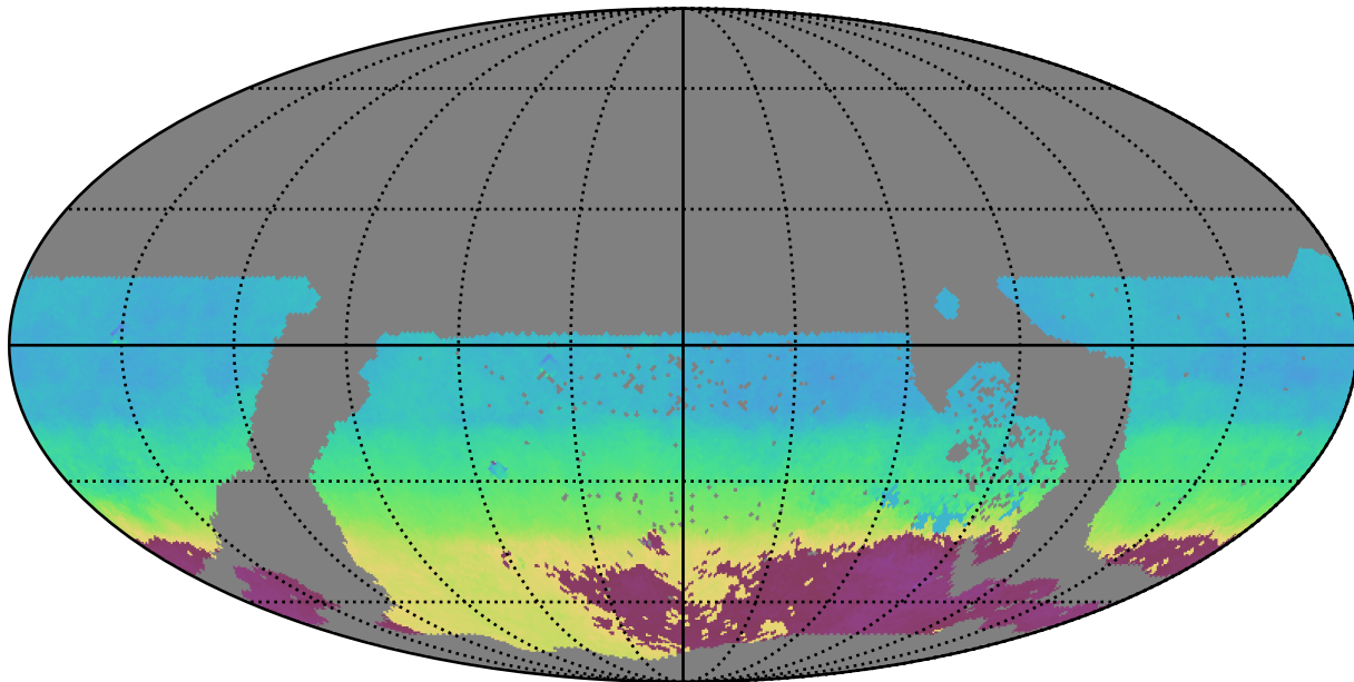
extra_ss_neo4_v3.4_10yrs WFD r band: AngleMean rotSkyPos
