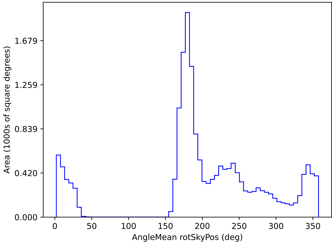
extra_ss_neo4_v3.4_10yrs WFD r band: AngleMean rotSkyPos
