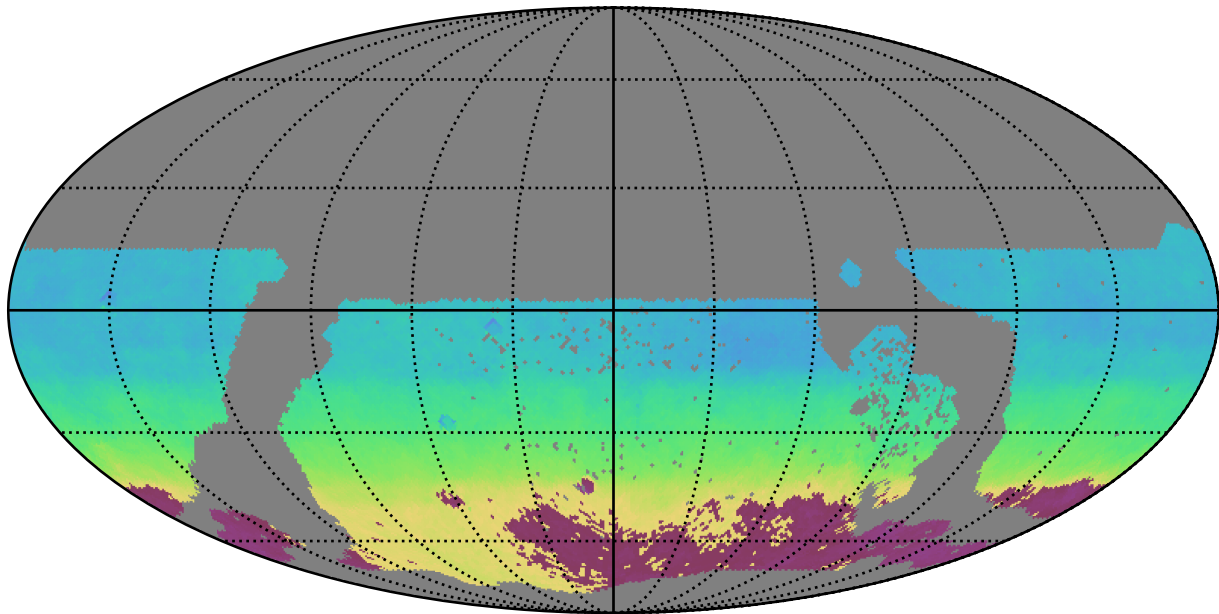
extra_ss_neo4_v3.4_10yrs WFD i band: AngleMean rotSkyPos
