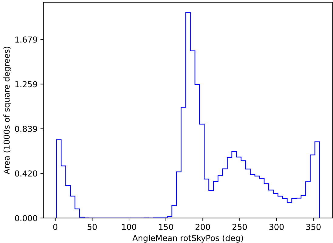
extra_ss_neo4_v3.4_10yrs WFD i band: AngleMean rotSkyPos
