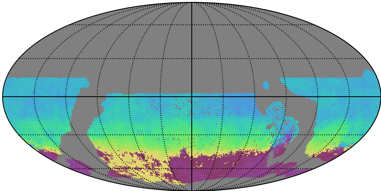
extra_ss_neo4_v3.4_10yrs WFD g band: AngleMean rotSkyPos
