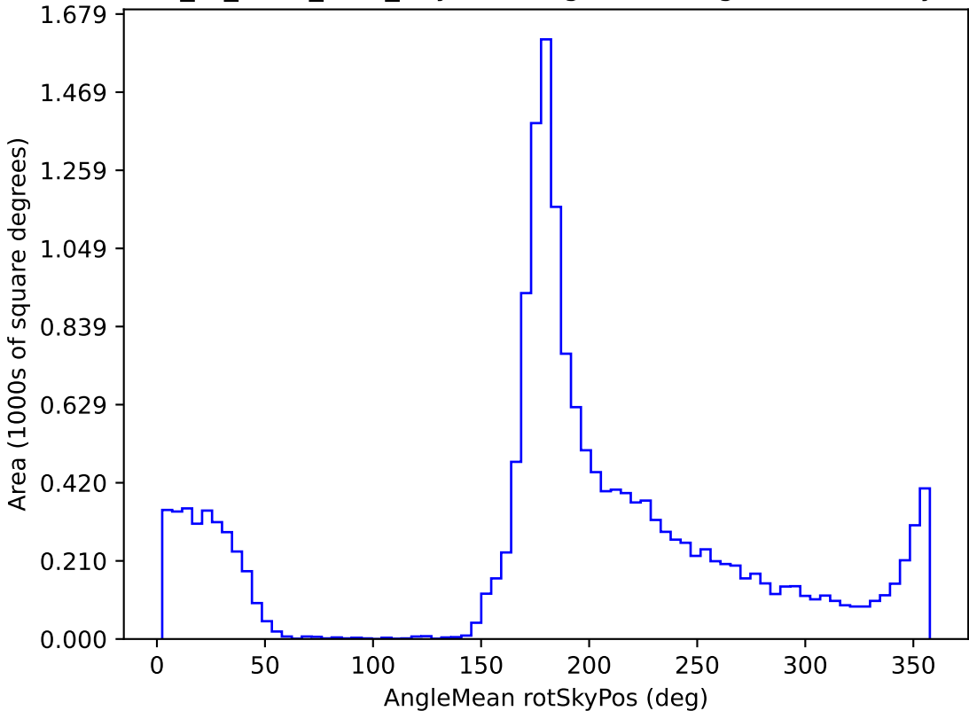
extra_ss_neo4_v3.4_10yrs WFD g band: AngleMean rotSkyPos
