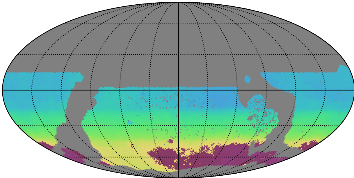
extra_ss_neo4_v3.4_10yrs WFD all bands: AngleMean rotSkyPos
